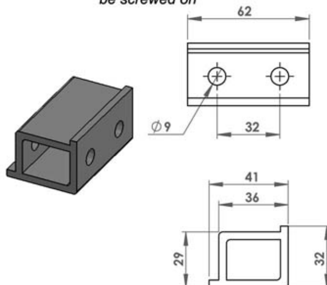
500 10 502 Gâche latérale zinguee à visser Side zinc plated steel keeper to be screwed on
