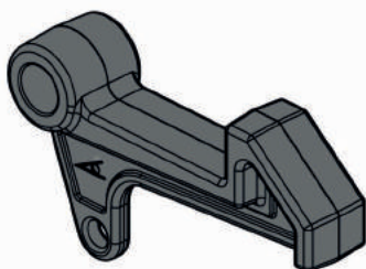
Crochet 26T - Hook 26T 500 00 067
